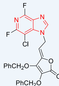
3-deazapurine 15
