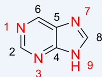
purine
